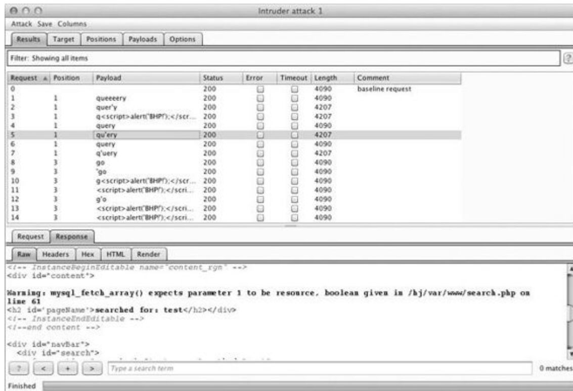
Figure 6-8. Our fuzzer running in an Intruder attack
